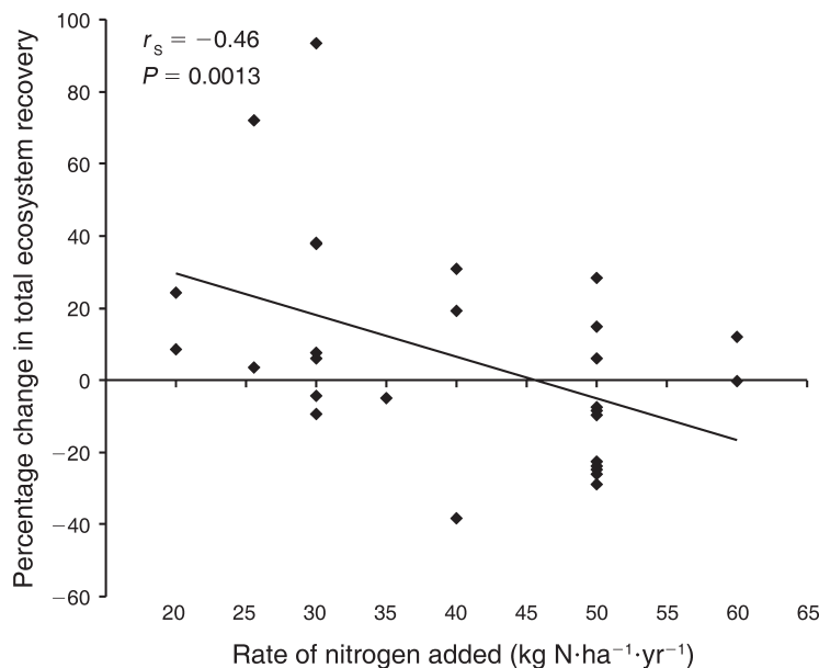
FIG. 6. Relationship between the percentage change in total ecosystem ^{15}\text{N} tracer recovery and the rate of N addition for all time periods. Positive values indicate greater total ecosystem ^{15}\text{N} tracer recovery following higher level of N addition. The Spearman rank correlation coefficient and P value are shown.
